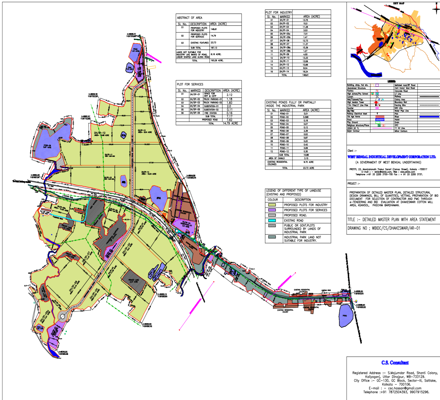
Master Plan of Dhakeswari Cotton Mill Premises
